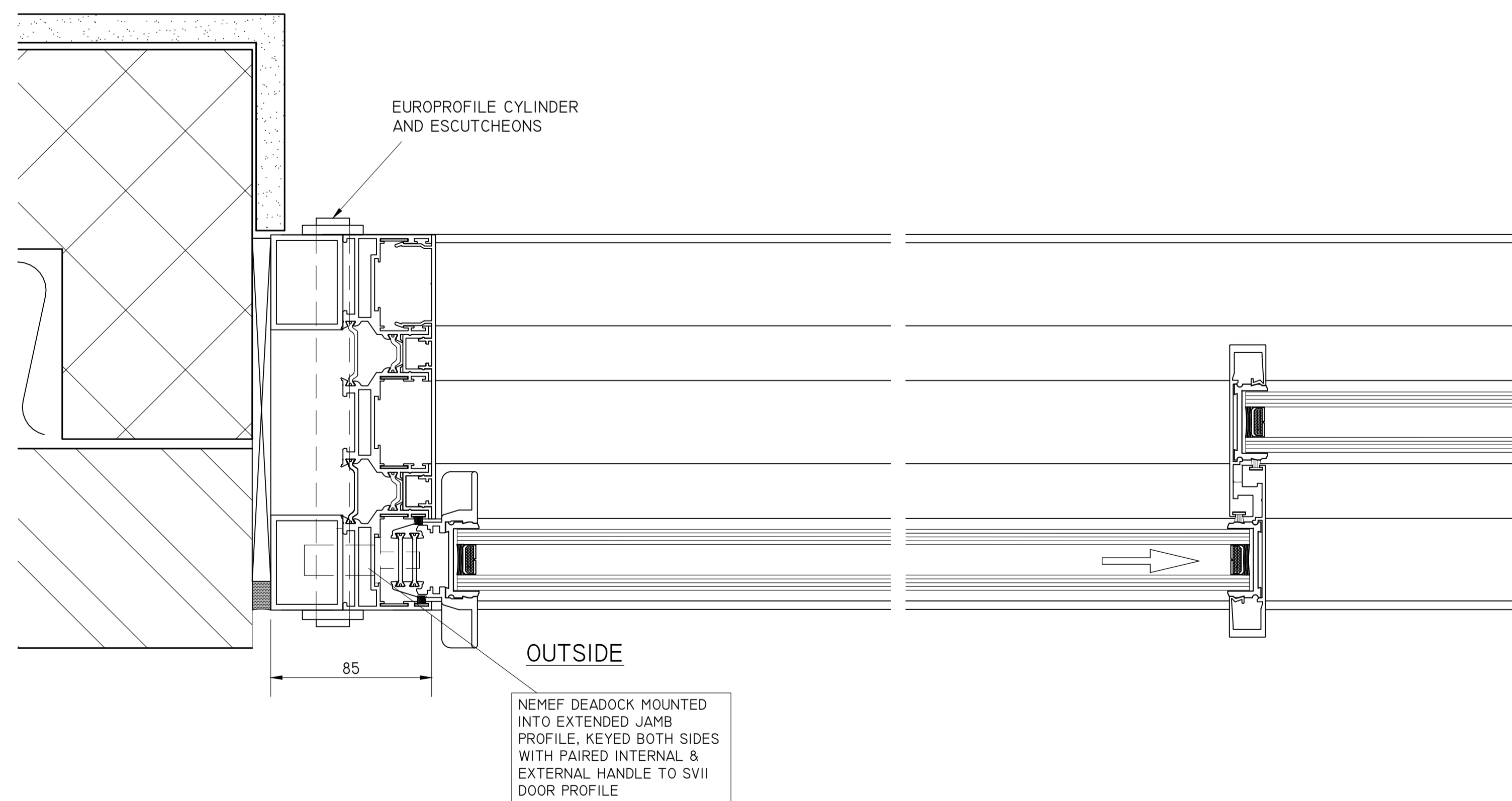
EXTERNAL LOCK JAMB DETAIL (3-TRACK)
