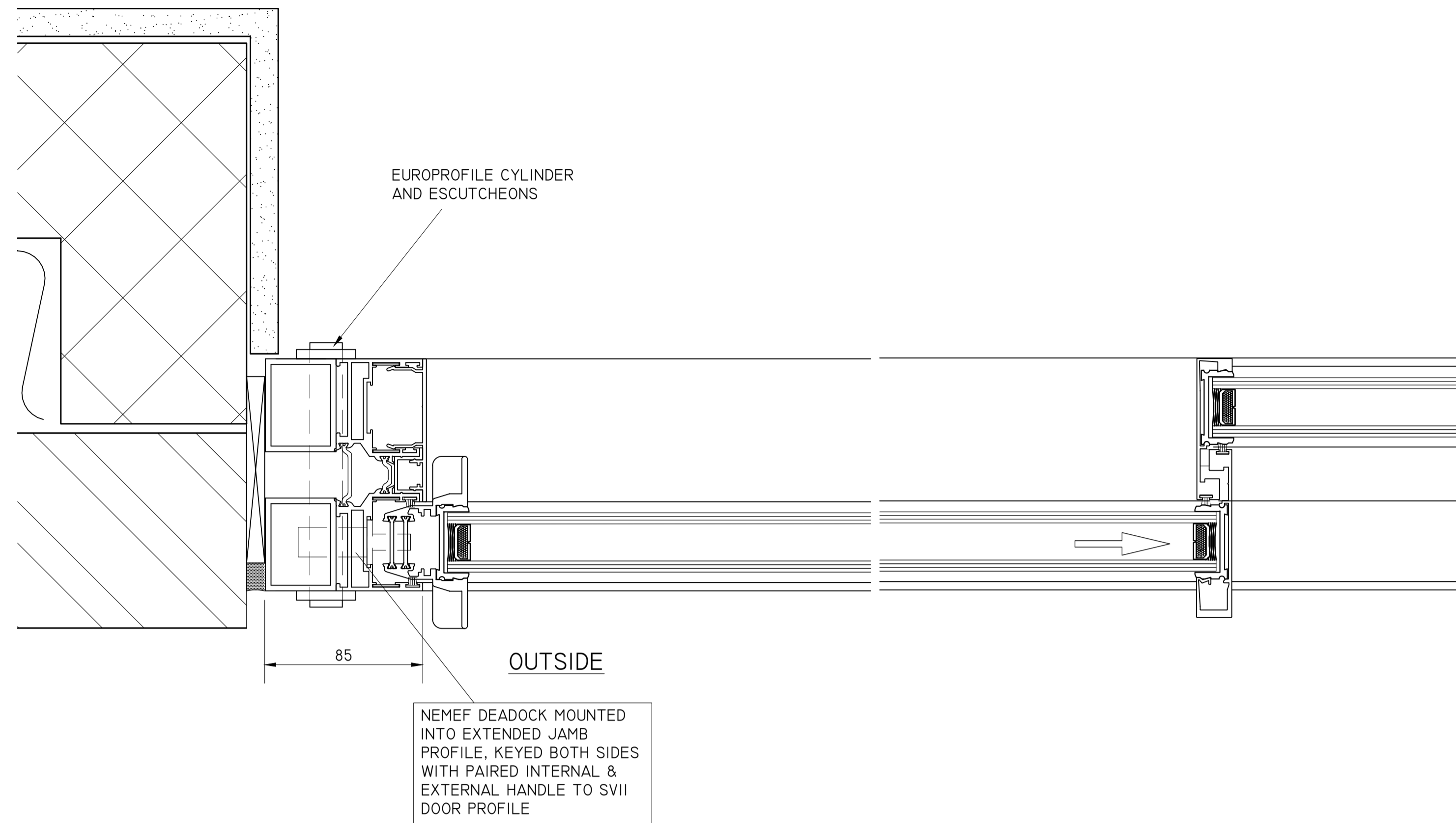
EXTERNAL LOCK JAMB DETAIL (2-TRACK)
